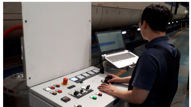
Step 4: After a retrofit with exchange of termination on the train, we recommend to perform a partial discharge test of the retrofit cable with EGT-75 to guarantee the quality of the assemble process.
